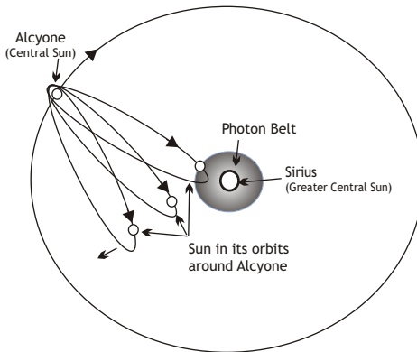
Sun in its orbits around Alcyone, occasionally entering the energy field of Sirius
