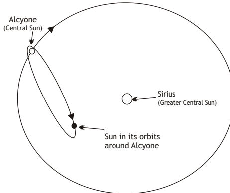
The Sun and Alcyone in their orbits
